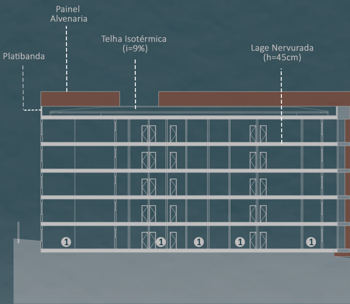
4 CORTE B - APT. ALUGUEL SOCIAL 0 5 15 1 10
